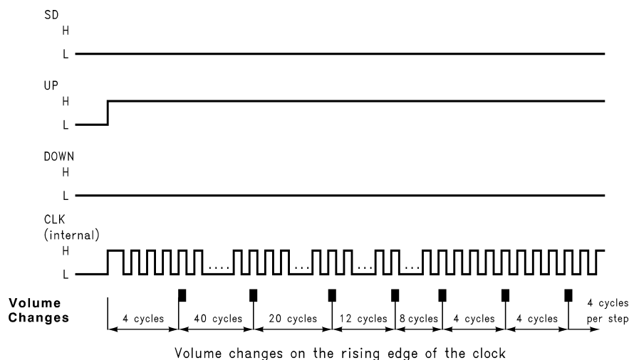
Figure 46. Volume Control Timing Diagram
