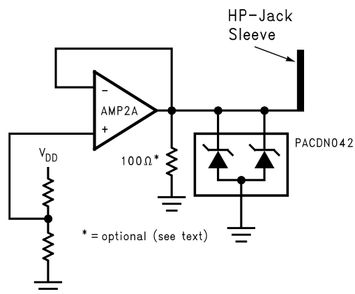
Figure 45. The PCDN042 provides additional ESD protection beyond the 2000V shown in the Absolute Maximum Ratings for the AMP2A output
